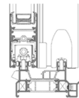
Cill Detail
