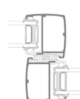
Interlock Detail
