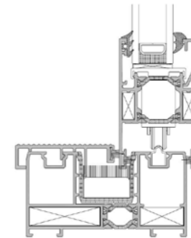
Cill detail
